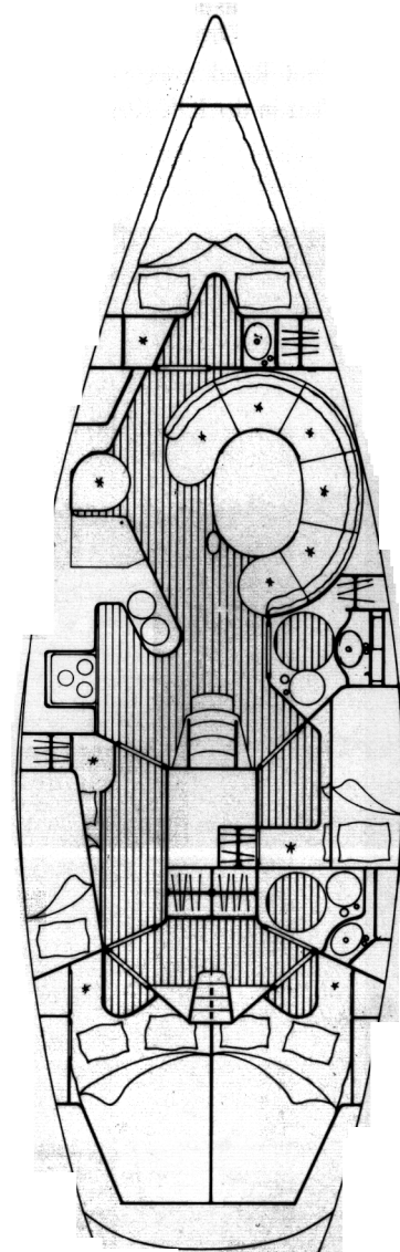
Charterversion with five cabins.
